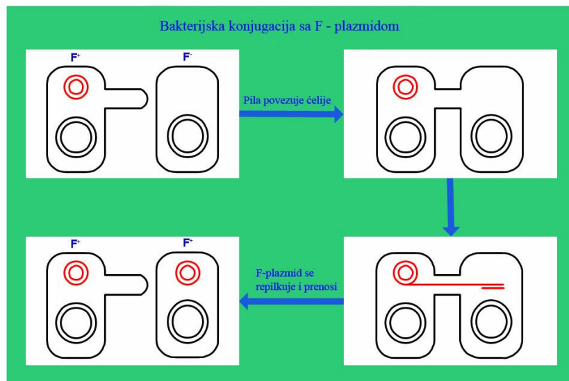
Slika 89. Konjugacija ( http://www.premedhq.com/2013/11/mcat-conjugation-and-mapping.html )
